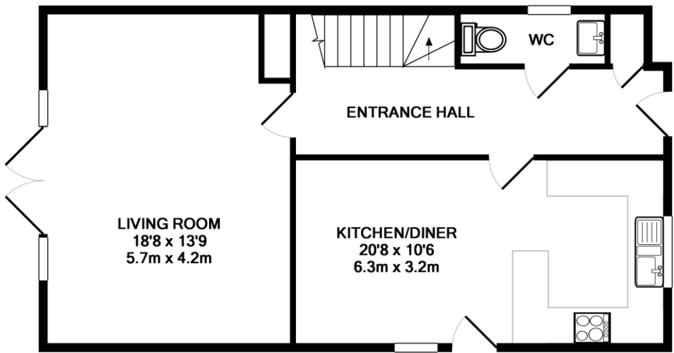
GROUND FLOOR APPROX. FLOOR AREA 59.3 SQ.M. (639 SQ.FT.)
